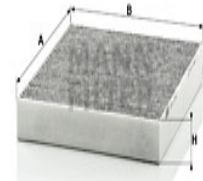
Cabin Air Filter CUK 2141 EM-40008
