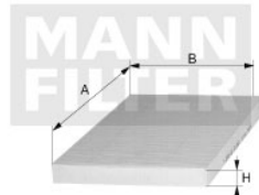
Cabin Air Filter FP-B02 EM-40102
